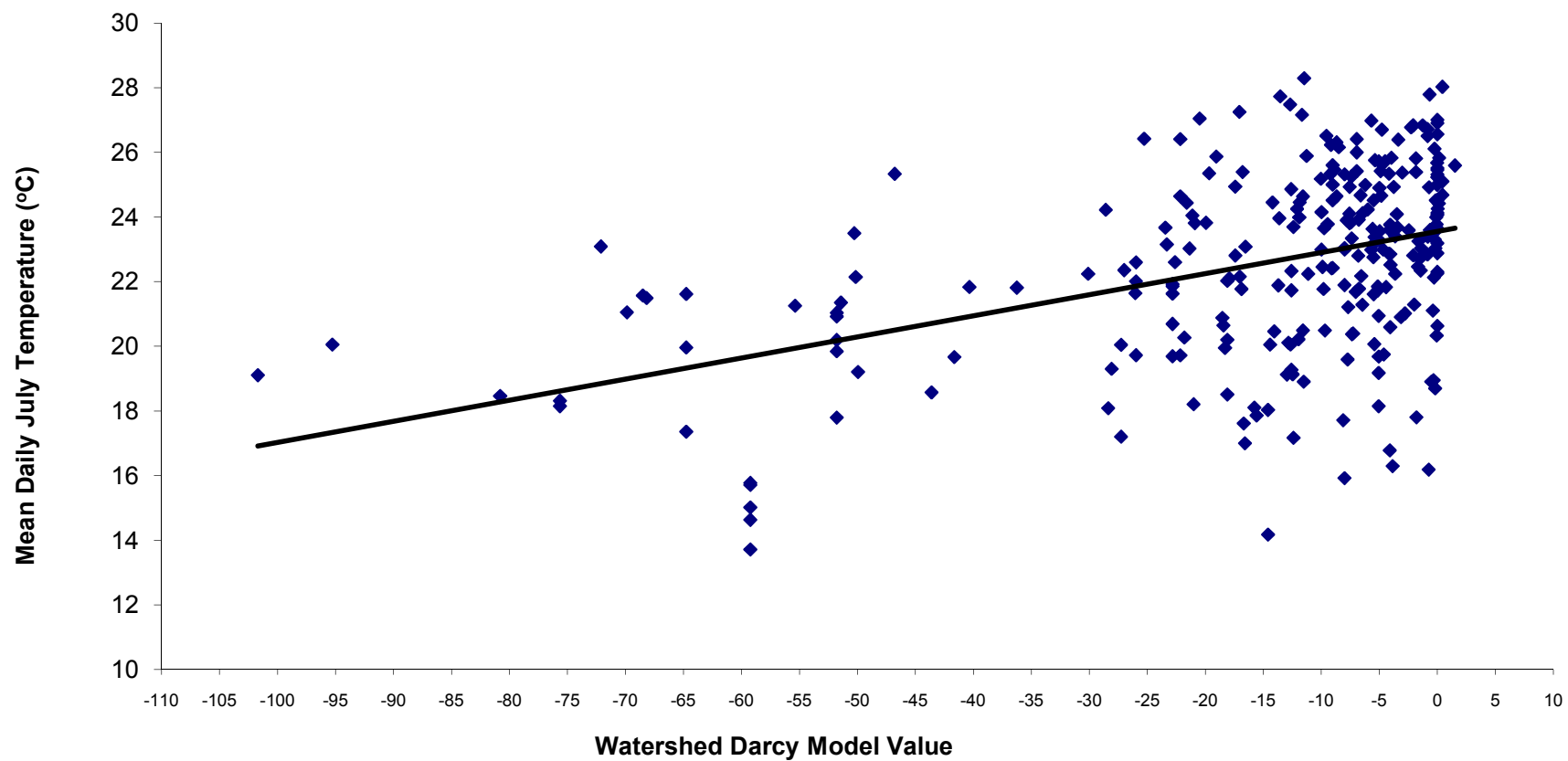
Figure 9. Comparison of measured temperature and modeled watershed Darcy value
