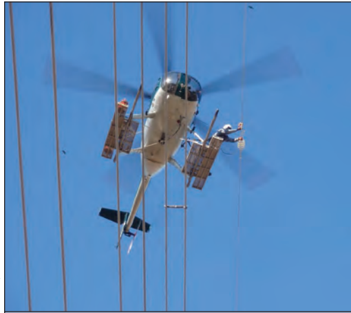
FIGURE 6.2: A helicopter crew installing line marking devices on a power line.
