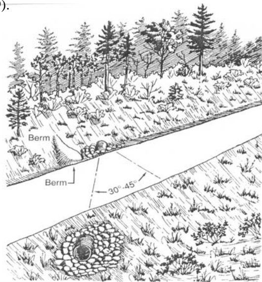
Figure 5-9. Cross-drain culvert.
