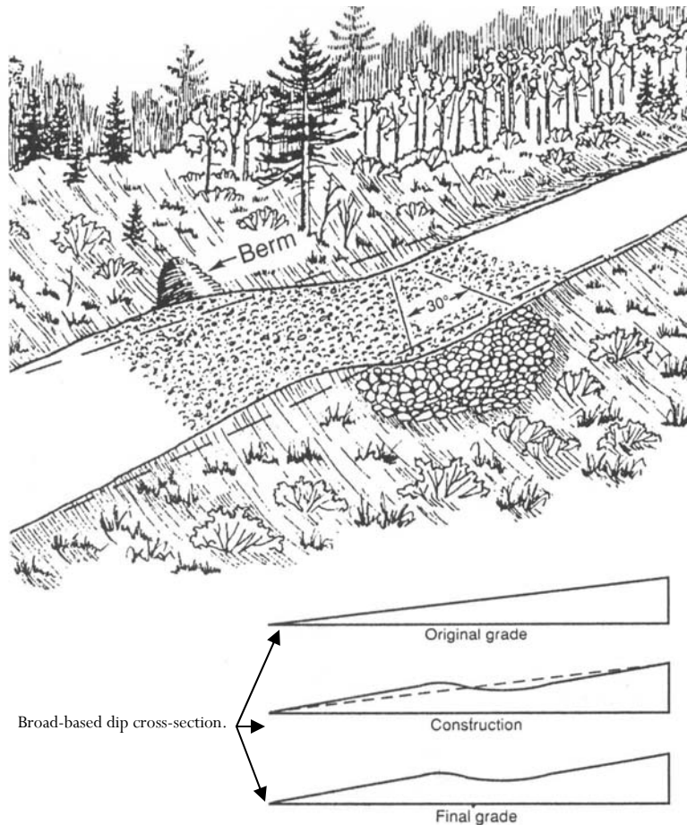
Figure 5-11. Broad-based dip.
