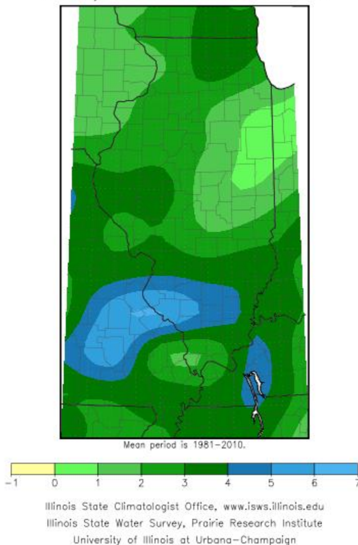
Figure 4. Precipitation Departure from Normal for Winter 2013.
