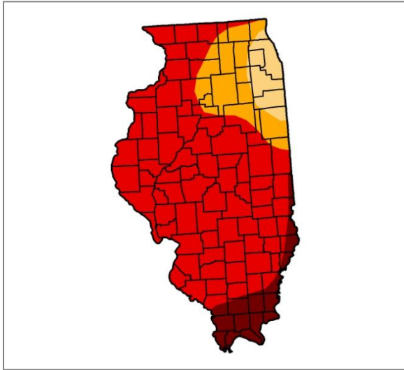
Figure 1. Monthly Drought Monitor continued
